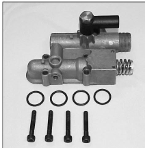
FA-YK157116600 Manifold Kit
